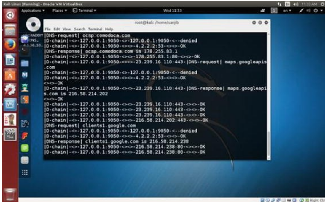
Figure 27-1. Tor is running through the terminal
